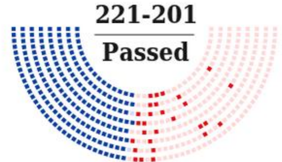
Seat position based on our ideology score .
